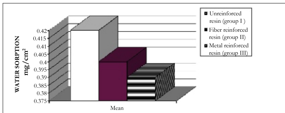
Figure 2. Shows the amount of water sorption (mg/cm 2 ) of unreinforced, fiber reinforced, and metal-filled resins.
