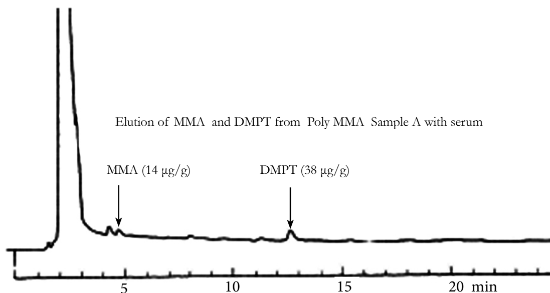
Figure 6. Elution of MMA and DMPT from PolyMMA samples A (Yunifast) and B (Acrom) into serum. The unit of MMA and DMPT amount is \mu\text{g}/\text{sample g} . No elution of DMPT was recognized in sample B Acron due to no use of DMPT for preparation.
