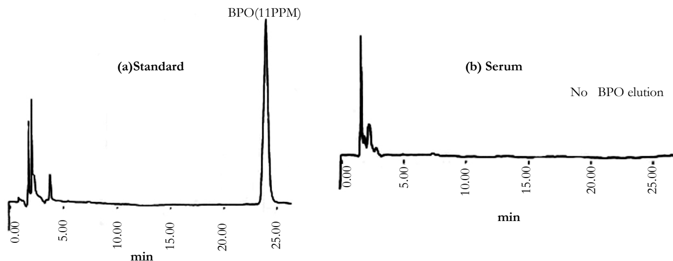
Figure 4. Solid phase extraction of BA transformed from BPO in serum using a C-18 column
