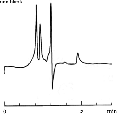
(4b) serum blank
