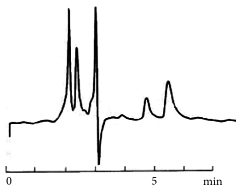
(4a) BA from BPO (2.2 ppm) in serum
